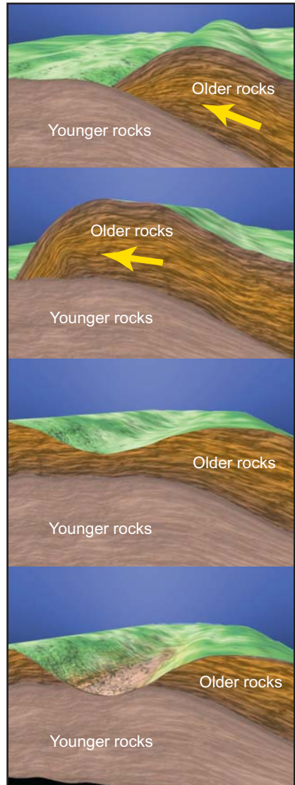
Figure 19. Stages in the development of a geologic window.
